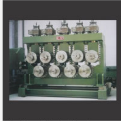
Section Straightening Machine
